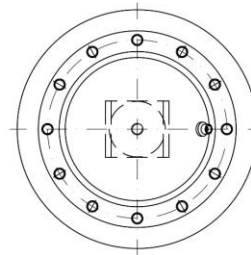
TOP VIEW (1:2)
